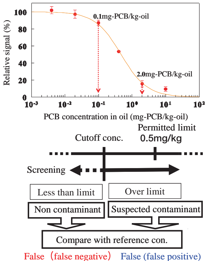
Fig.1 Dynamic range of PCB concentration in oil (Left).
